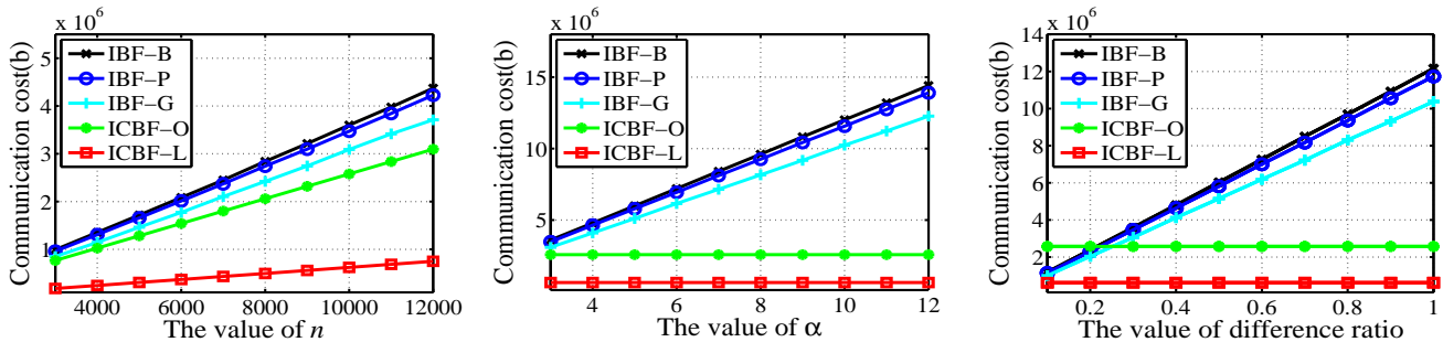
(a) Communication overhead when n varies. (b) Communication overhead when \alpha varies. (c) Communication overhead when d/n varies. Fig. 6. The communication overhead of IBF and ICBF for multiset synchronization with different parameter settings. Apparently, unlike IBF, ICBF is insensitive to \alpha or d , but is only decided by the maximum number of elements in the root sets.
