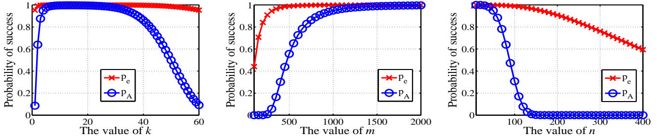
(a) Impact of k when m=1000, n_A=50 . (b) Impact of m when n_A=50, k=4 . (c) Impact of n_A when m=1000, k=4 . Fig. 3. The changing trends of successful representation probability of an element ( p_e ) and the entire multiset ( p_A ), with different parameter options.
