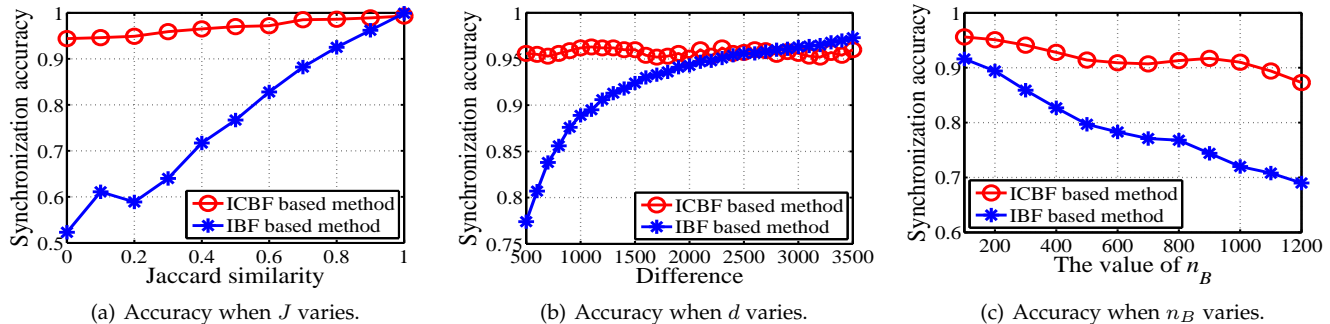
Fig. 4. The synchronization accuracy of ICBF and IBF under different parameter settings.
