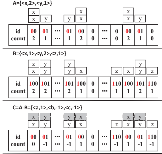
Fig. 2. An example of ICBF encoding and subtracting process with A=\langle x,2\rangle,\langle y,1\rangle and B=\langle x,1\rangle,\langle y,2\rangle,\langle z,1\rangle .
