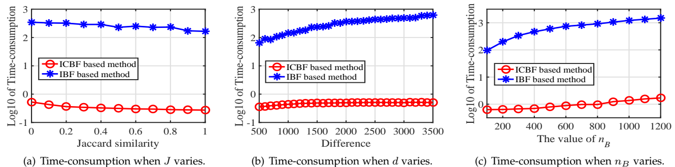
Fig. 5. The time-consumption of ICBF and IBF under different parameter settings.
