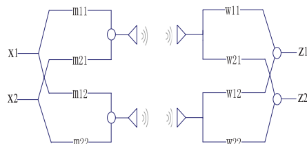
Fig. 1. An example of MIMO processing.
