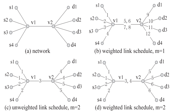
Fig. 5. An illustrative example: unweighted link schedule is inefficient.
